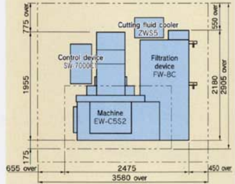
< Layout Diagram >
